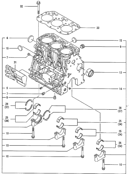
Fig.1. CYLINDER BLOCK
