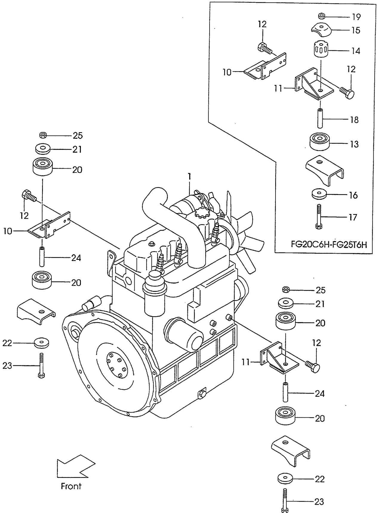
Fig.1 ENGINE MOUNT (F5H21010)
