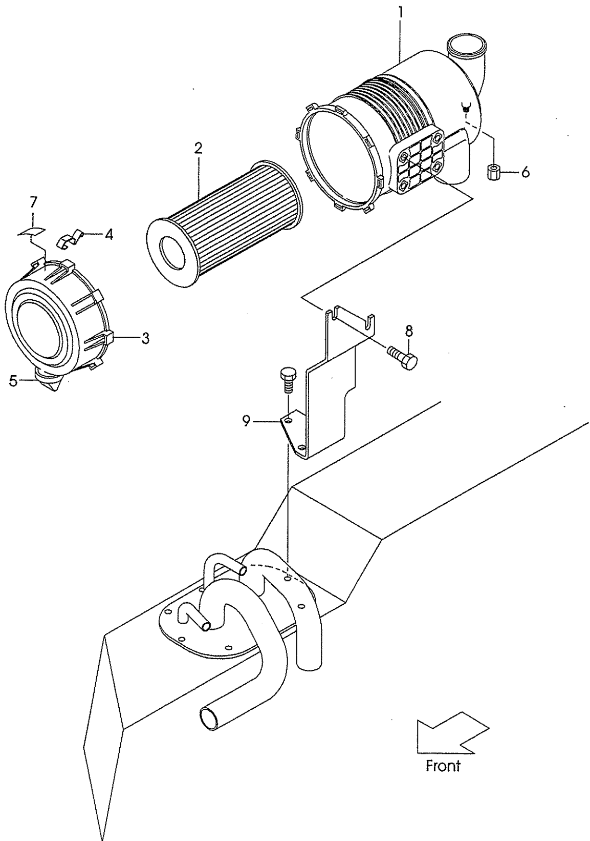
Fig.3 AIR CLEANER (G-TYPE) (F5H11030)
