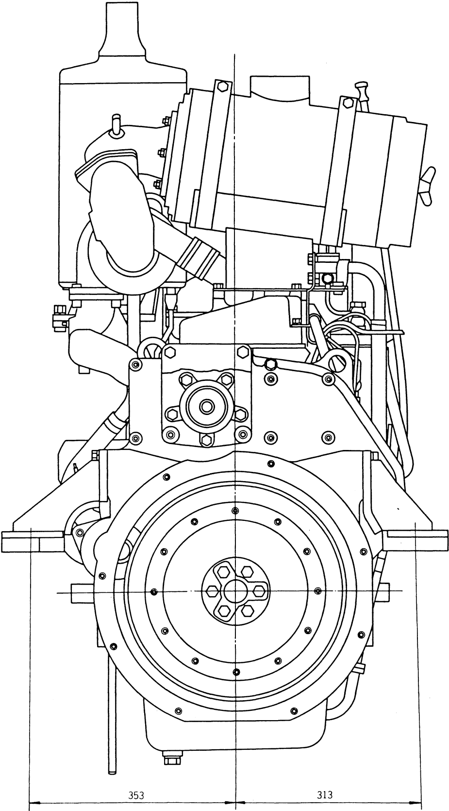
S4D105-3 REAR VIEW (For D45A, P-1)
