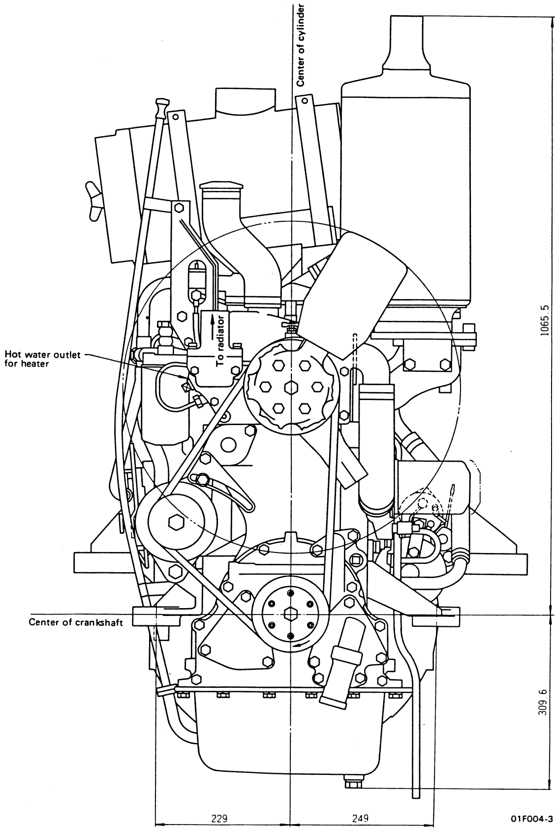
S4D105-3 FRONT VIEW (For D45A, P-1)
