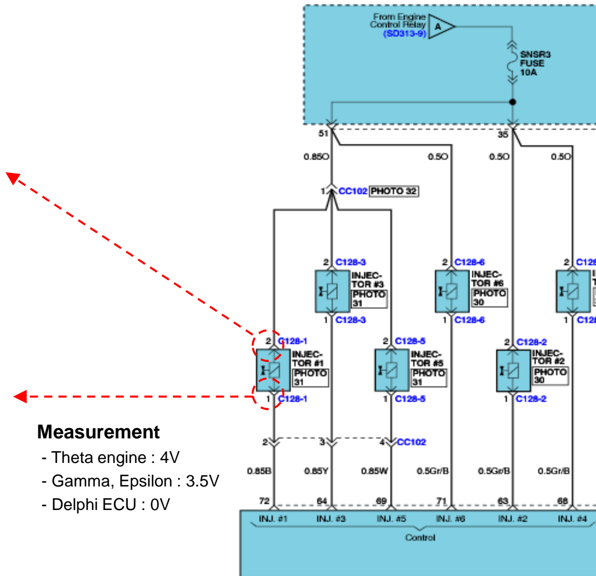
[Wiring inspection-power supply]
