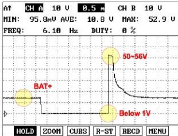
[Injection waveform]
