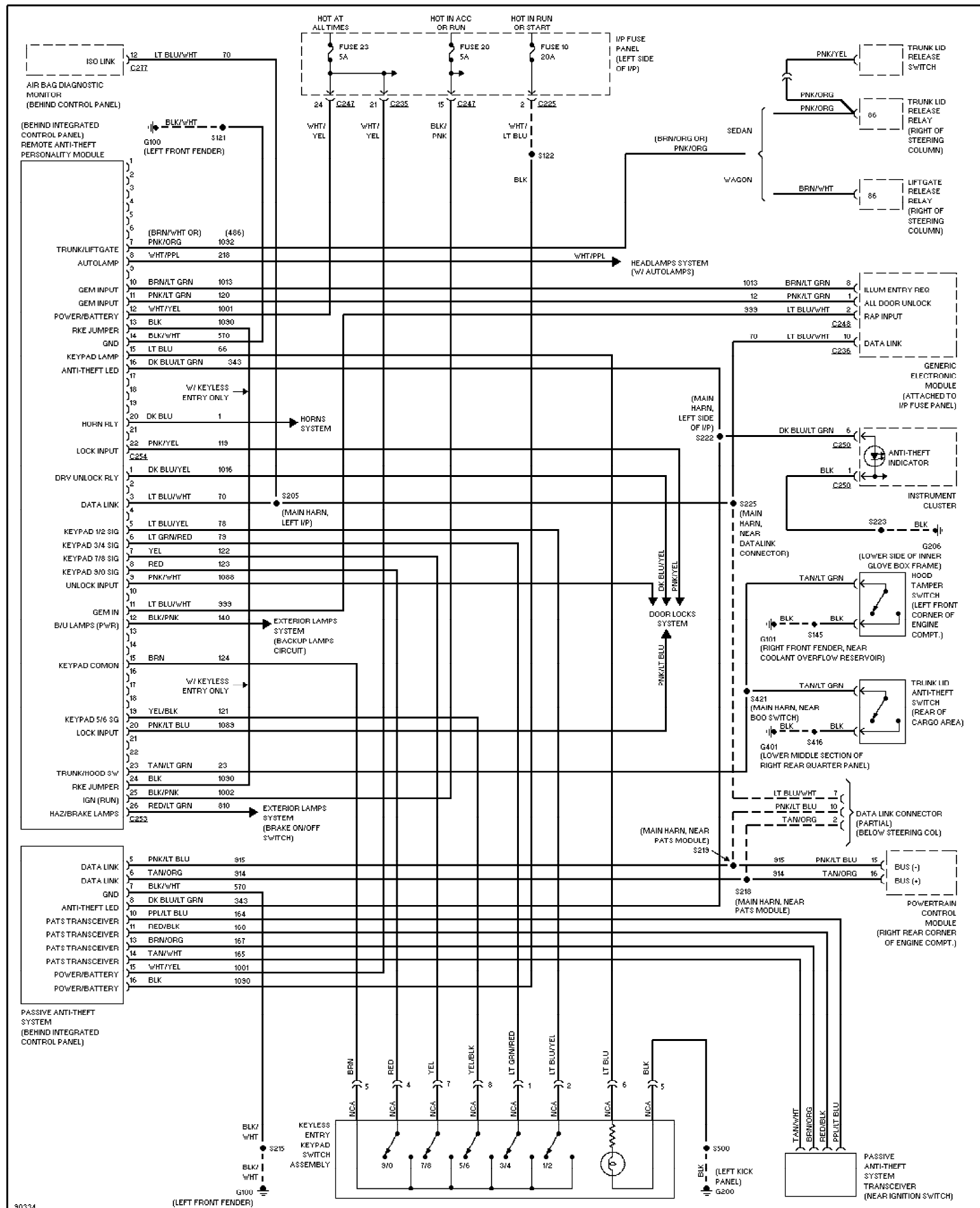
Fig. 4: Anti-theft Circuit 1997 Ford Taurus LX
