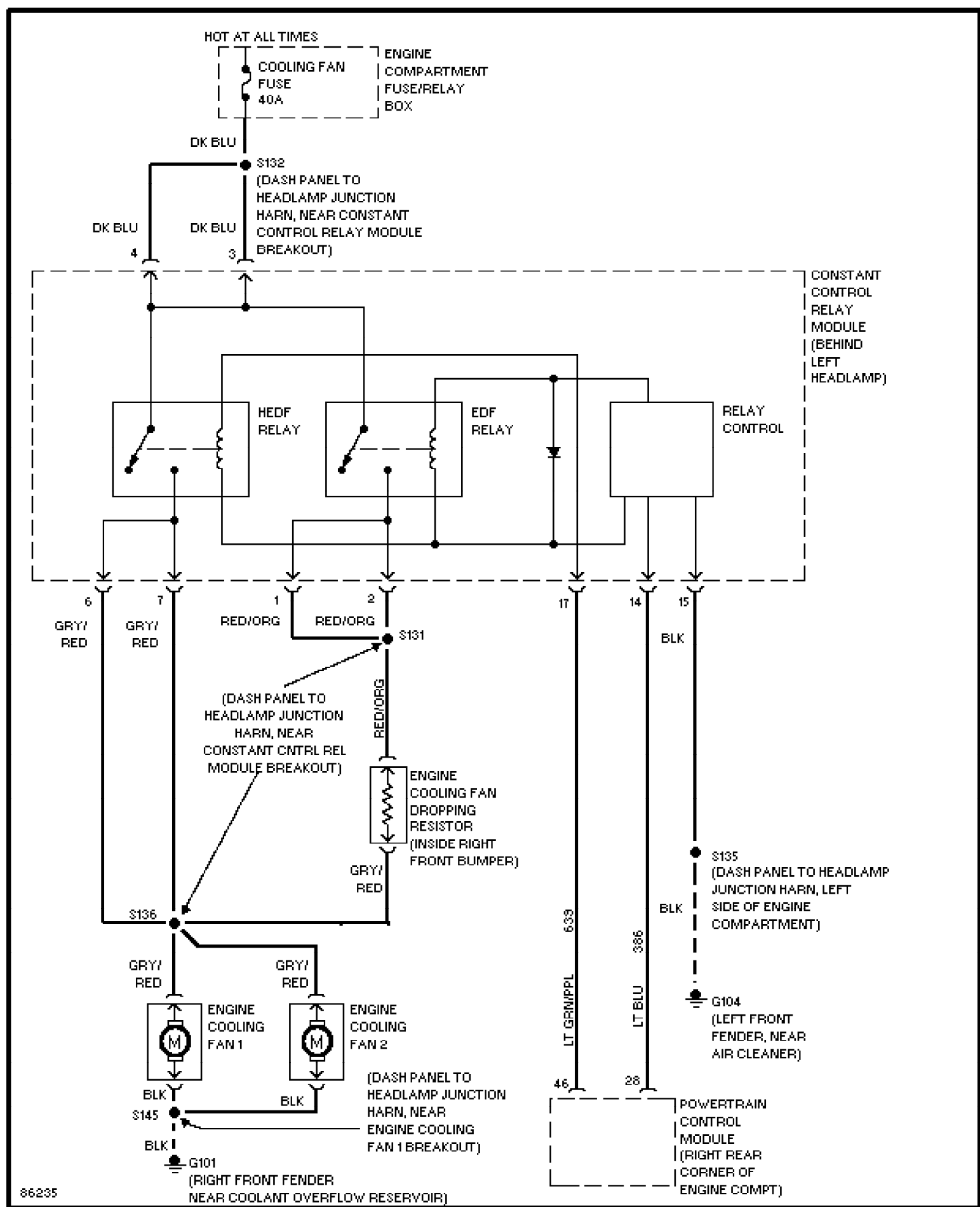
Fig. 7: Cooling Fan Circuit 1997 Ford Taurus LX
