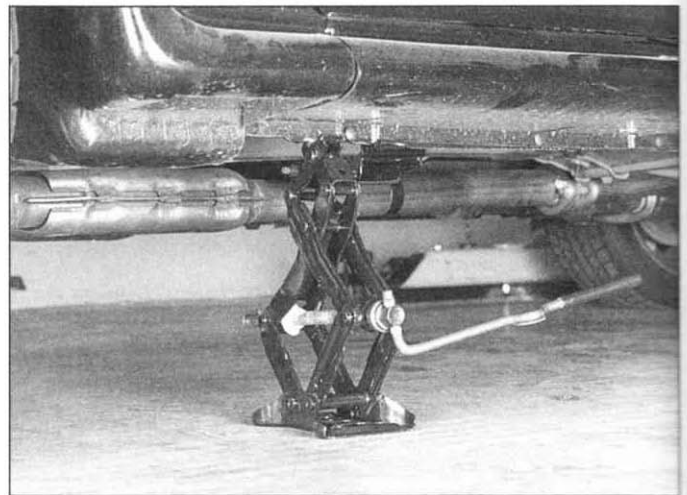
Place the jack so it engages the notch in the rocker panel nearest the wheel to be raised
