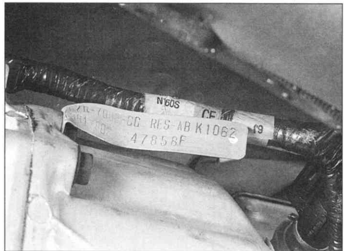
The manual transmission identification tag is retained by a left side engine-to-bellhousing bolt
