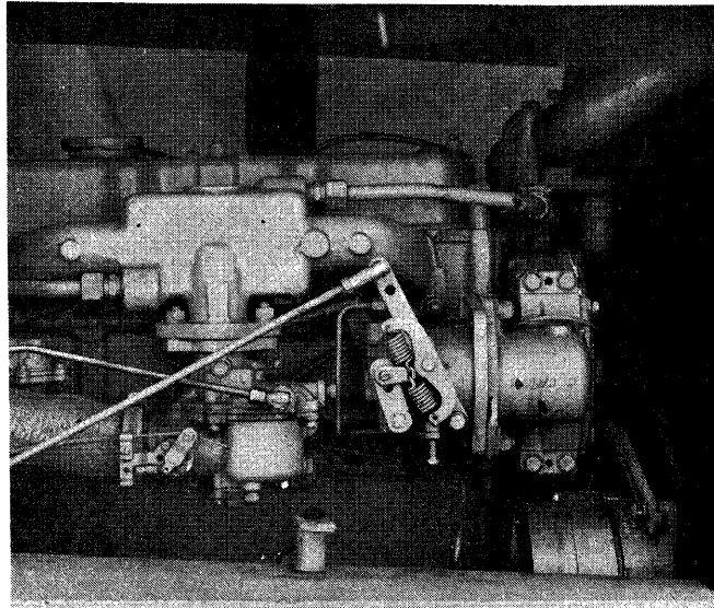
GAS ENGINE SERIAL NUMBER BEHIND GOVERNOR
